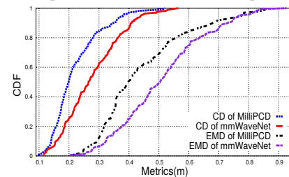
Figure 2: CDF for quantitative performance
