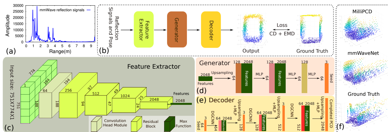
Figure 1: (a) Example of mmWave reflection signal; (b) mmWaveNet architecture overview; (c) Architecture of Feature Extractor; (d) Generator architecture; (e) Decoder architecture; (f) Output of MilliPCD and mmWaveNet comparing with ground truth PCD.
